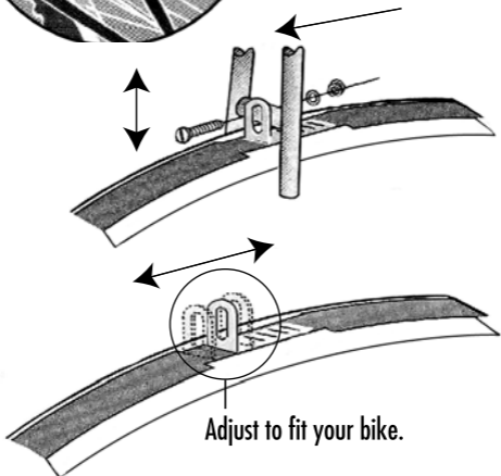
Rear fender
